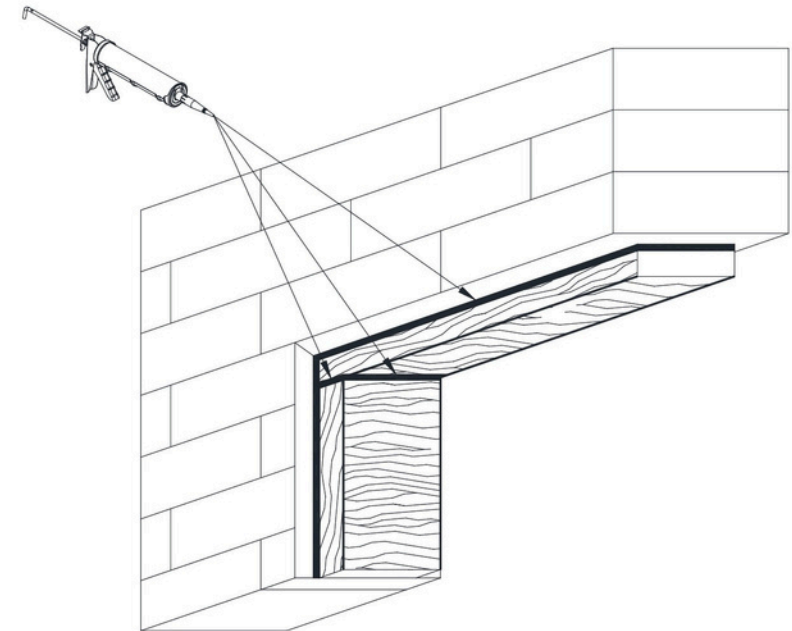
Wood buck seal
